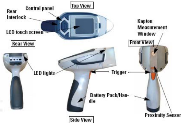
Figure 0-1. Analyzer Overview
