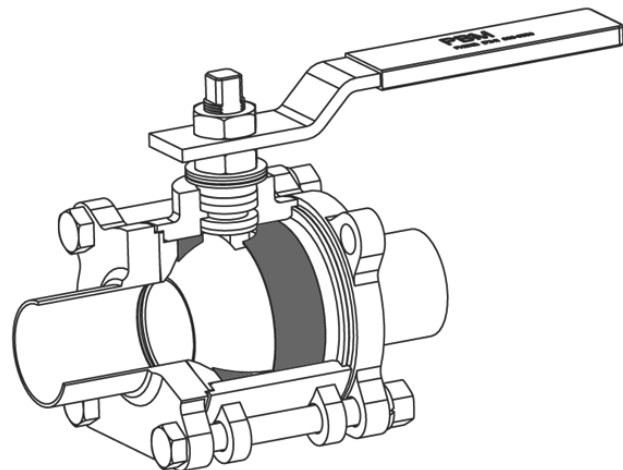
Cavity Fillers
