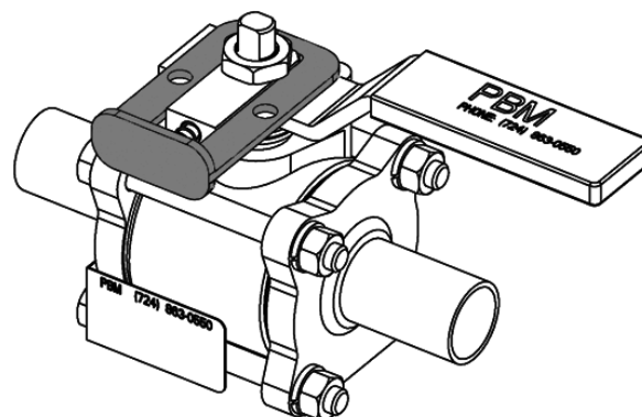
Locking Handle
