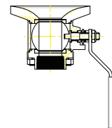
Straight Stem Flush Tank Ball Valve (FT)
