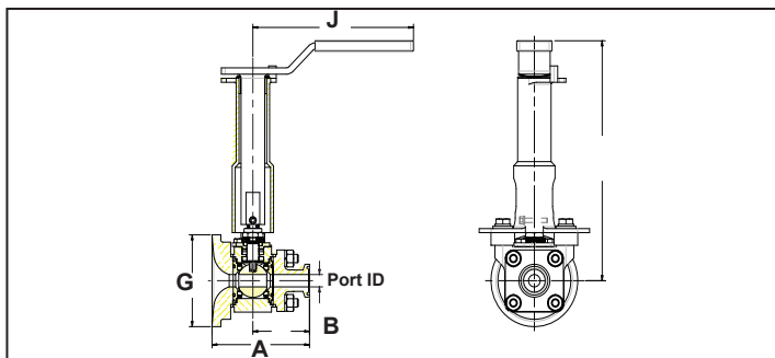
Flush Tank Valve with Extended Locking
