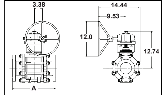
2-Way Valve with Gear Operator (6" only)
